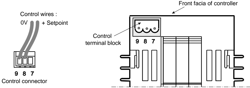
Figure 3-2 Control terminal block (view from below)
