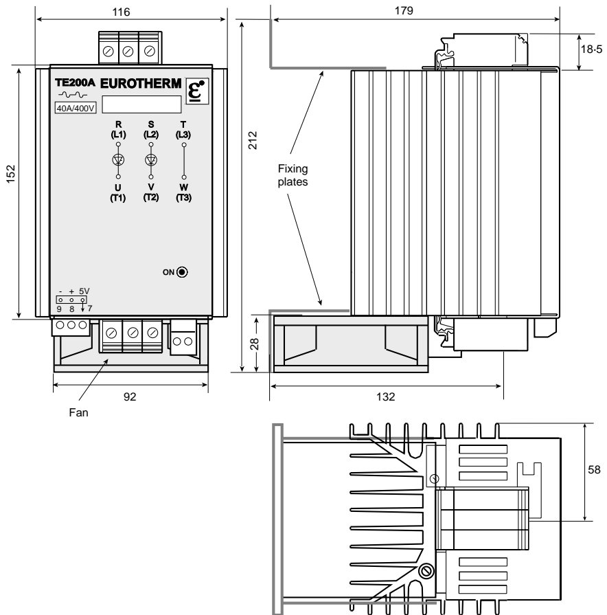
Figure 2-2 Dimensions (mm) of fan-cooled TE200A controller (63A rating)
