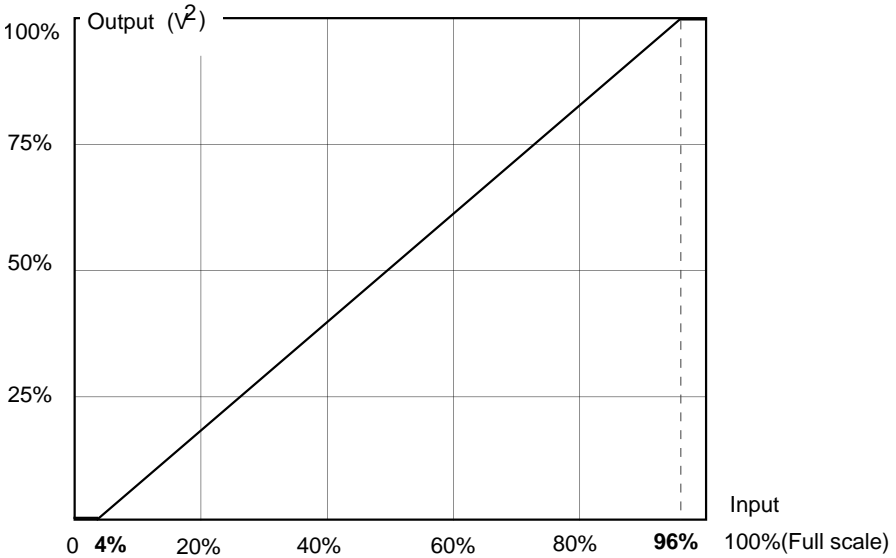
Figure 5-4 'Input/Output' response curve
