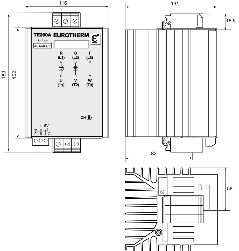
Figure 2-1 Dimensions (mm) of non fan-cooled TE200A controller
